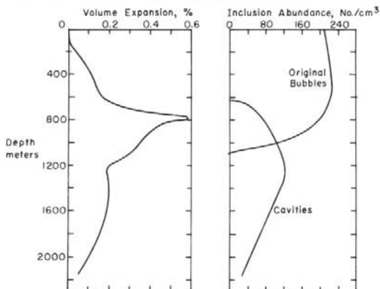
Figure 5. Relationship of relaxation trends (volume expansion based on density measurements) to bubble and cavity abundances measured 16 months after ice cores were drilled at Byrd Station, Antarctica. (Adapted from Gow (1971)).
