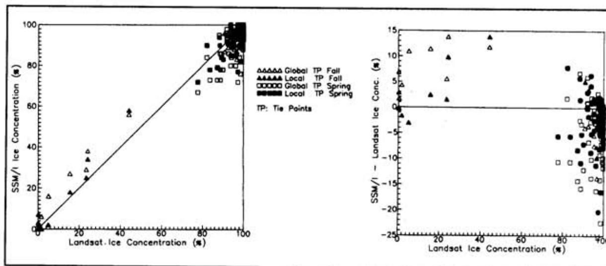
Figure 1. Comparison of ice concentration (50 km grid) between NASA Team Algorithm using local and global tie points versus Landsat values for the Beaufort, Chukchi, Weddell and Greenland seas, spring and fall conditions.
