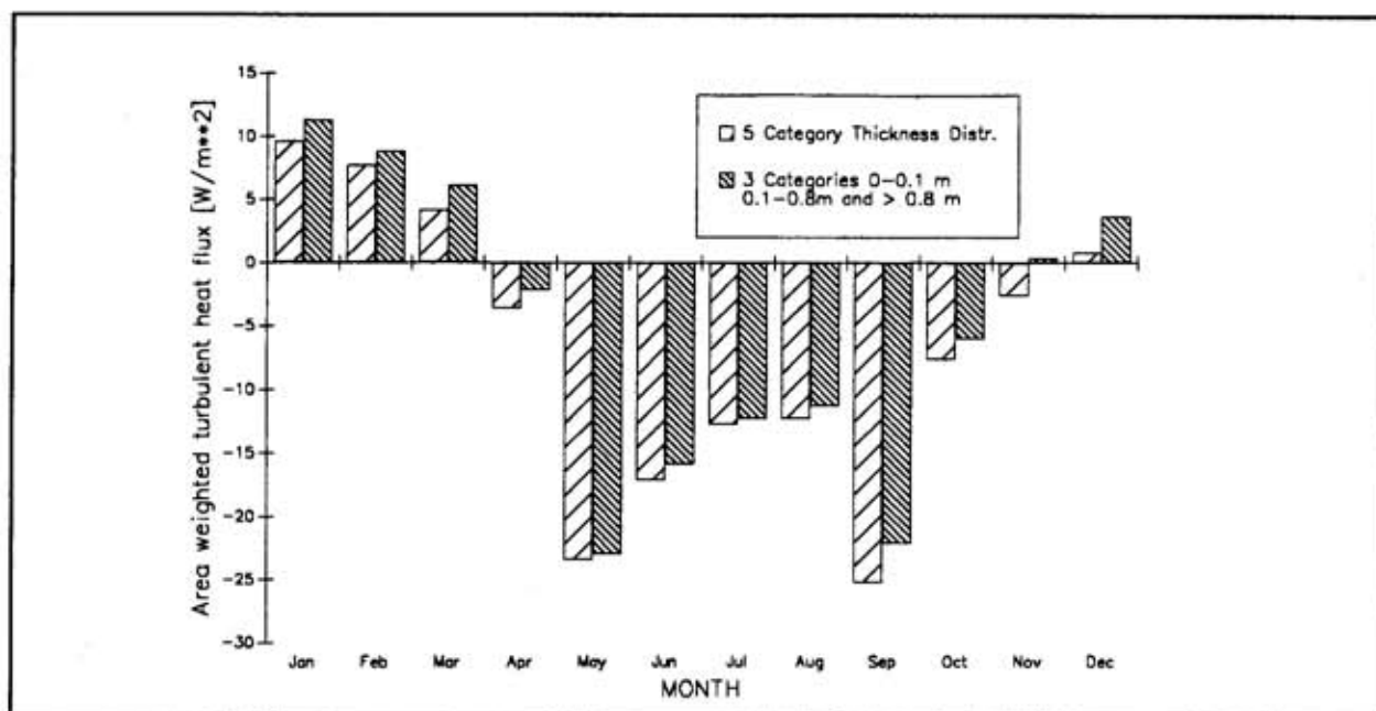
Figure 5. Turbulent heat fluxes [ \text{Wm}^{-2} ] calculated for a 5 category (0-0.1, 0.2, 0.4, 0.8, > 0.8m) and 3 category (0-0.1, 0.8, >0.8 m) thickness distribution.
