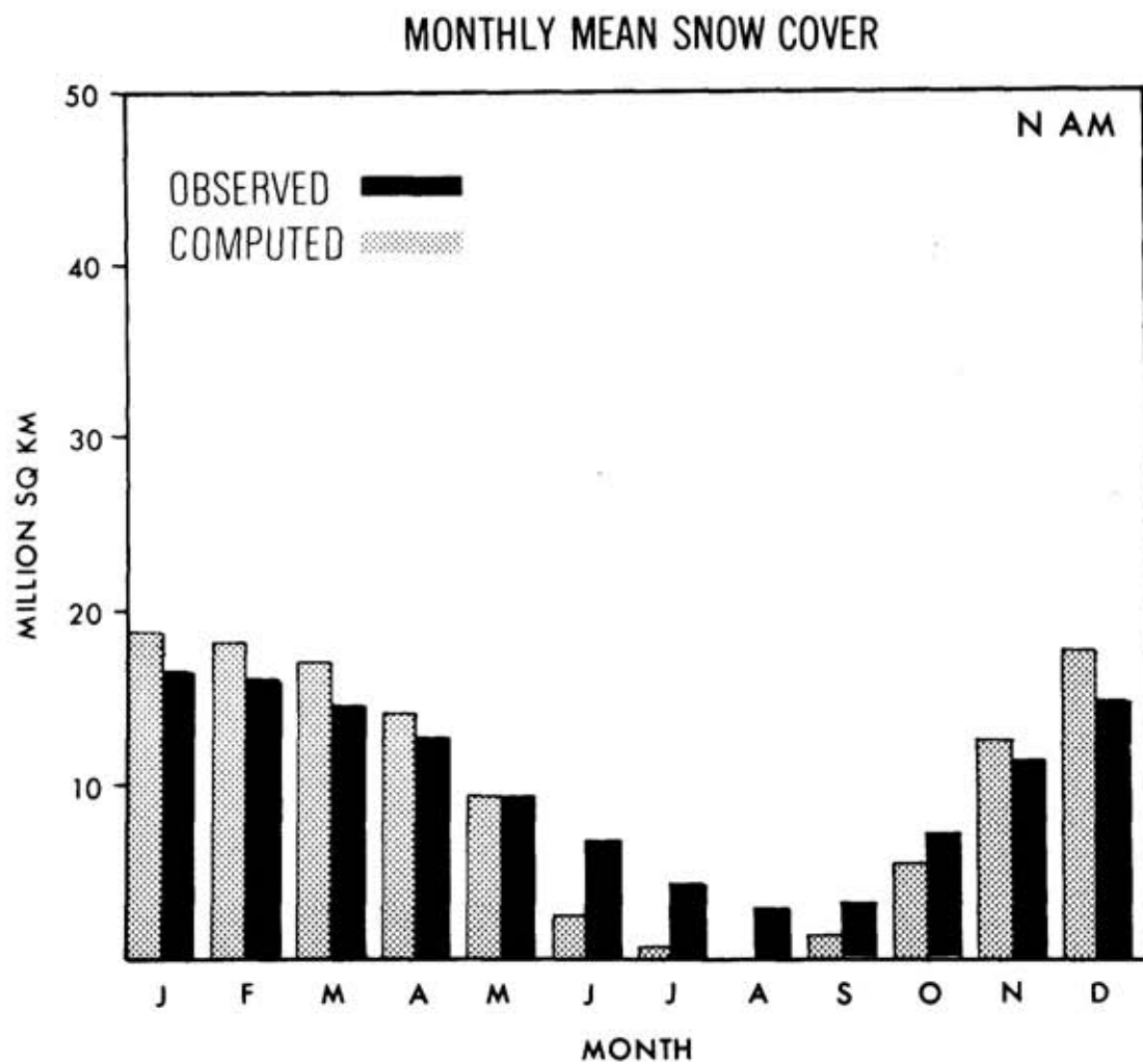
Figure 3. Monthly mean snow cover for North America as observed (Matson, personal communication) and as computed by the GCM.
