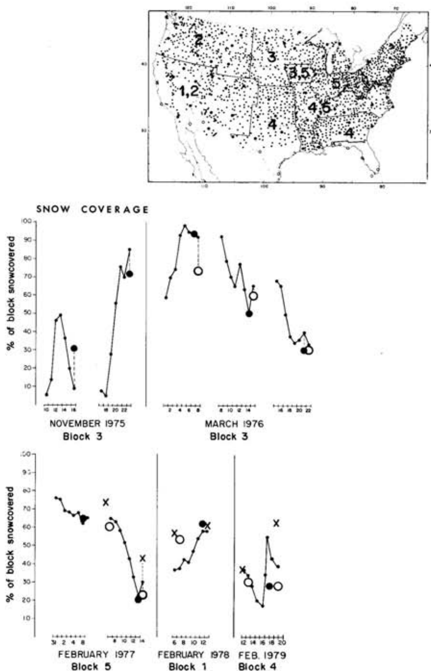
Figure 2. Snow coverage, in percent of total area, of selected U.S. geographic blocks. Blocks, some overlapping, are shown in the upper right. Daily data obtained from Lamont charts are shown by dots; area in the weekly NOAA/NESS snow chart is shown by a full circle plotted on the last day of the charted week; areas from the Weekly Weather and Crop Bulletin are shown by an open circle; and areas in the Air Force charts are shown by a cross.
