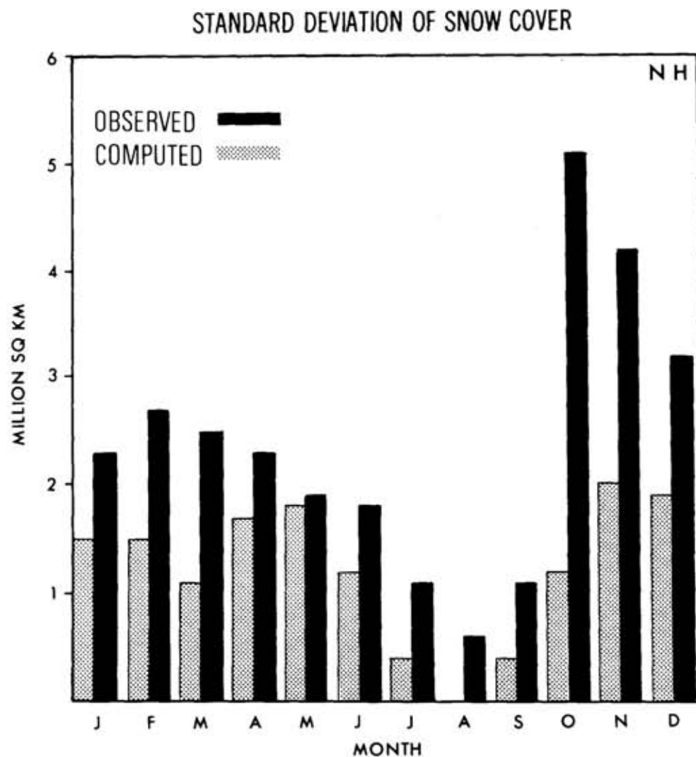
Figure 4. Standard deviation of monthly mean snow cover of the Northern Hemisphere as observed (Matson, personal communication) and as computed by GCM.
