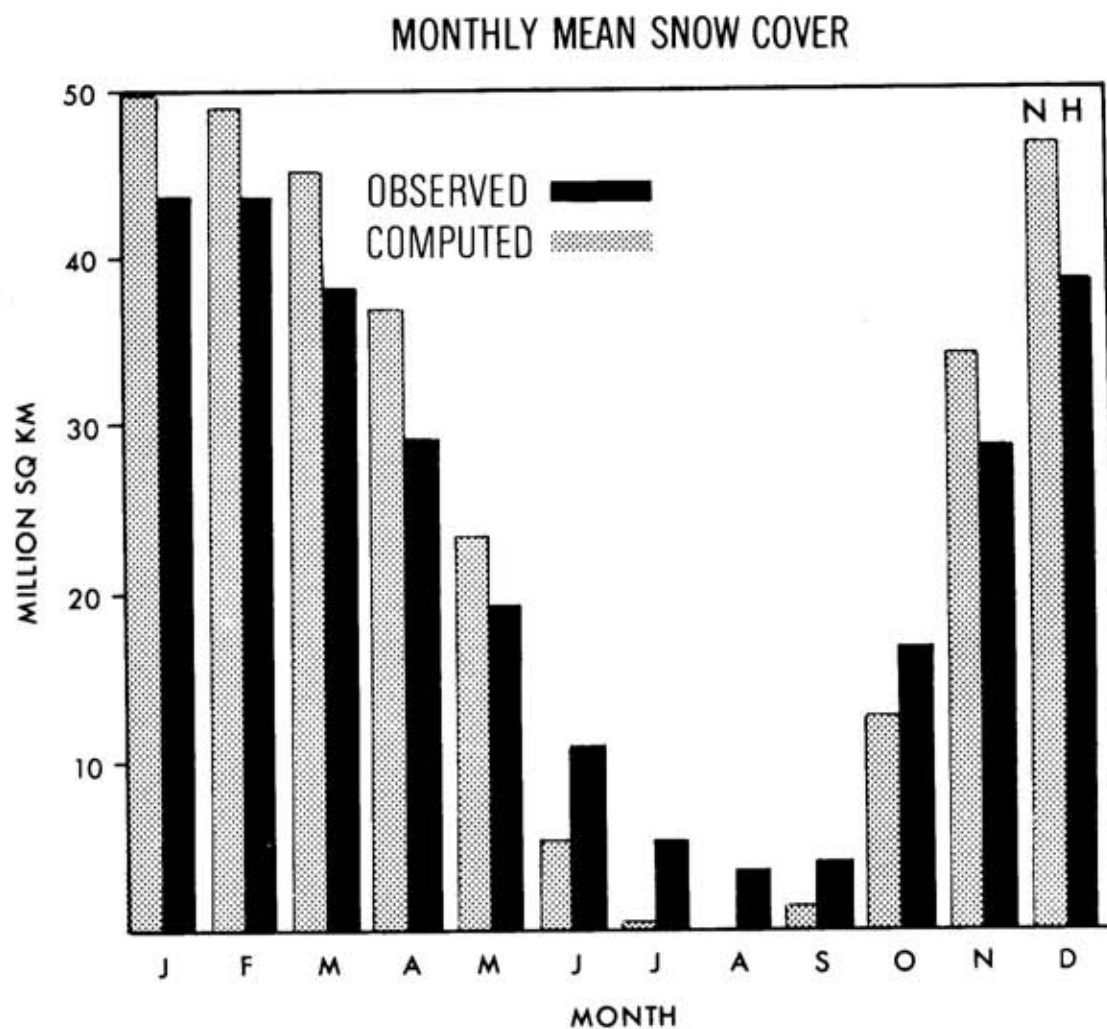
Figure 1. Monthly mean snow cover for the Northern Hemisphere as observed (Matson, personal communication) and as computed by the GCM.
