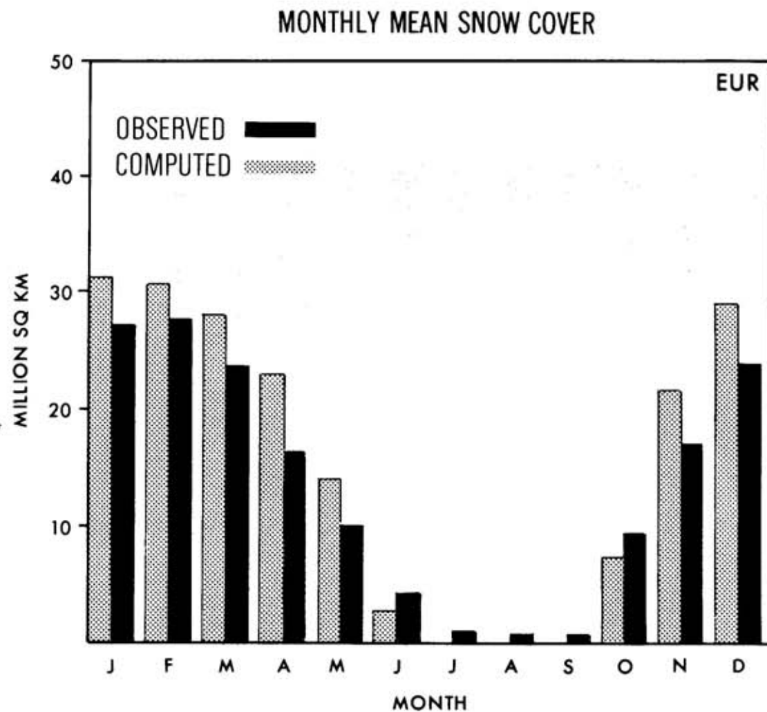
Figure 2. Monthly mean snow cover for Eurasia as observed (Matson, personal communication) and as computed by the GCM.
