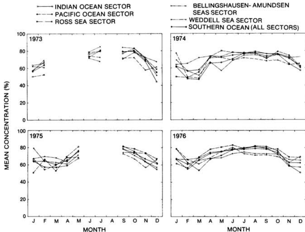
Figure 10. Mean ice concentration as a function of season for individual sectors during 1973-1976.
